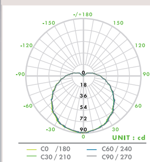
LUMINOUS / CANDLE POWER DISTRIBUTION
