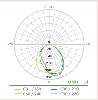
LUMINOUS / CANDLE POWER DISTRIBUTION
